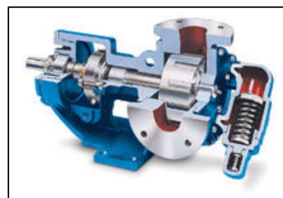
Figure 1. Internal gear pumps are ideal for high-viscosity liquids, but they are damaged when pumping large solids.
