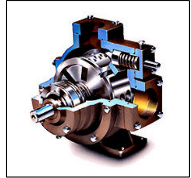
Figure 4. Vane pumps have better dry priming capability than other positive displacement pumps.
